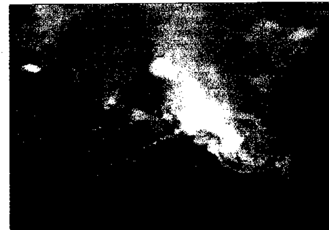
Photo Left - Recent Eruption of Mt. Pago on
